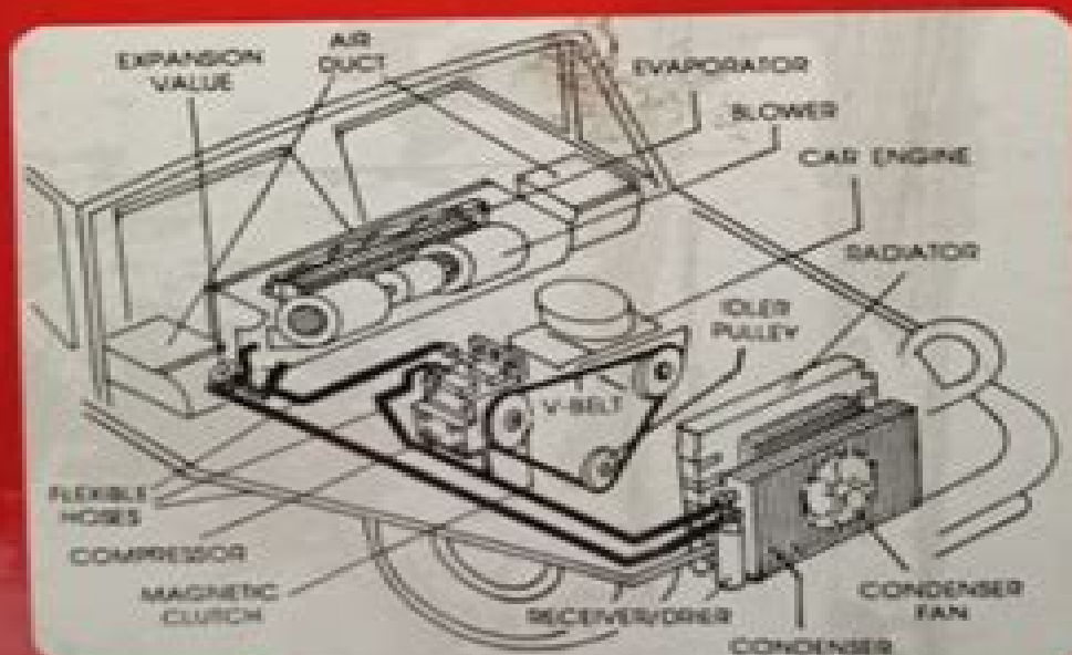
AUTOMOTIVE AIRCONDITIONING SYSTEM
