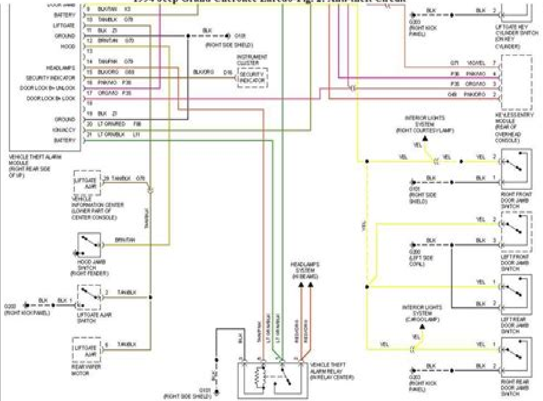
1994 Jeep Grand Cherokee Laredo-Fig. 2: Anti-theft Circuit
