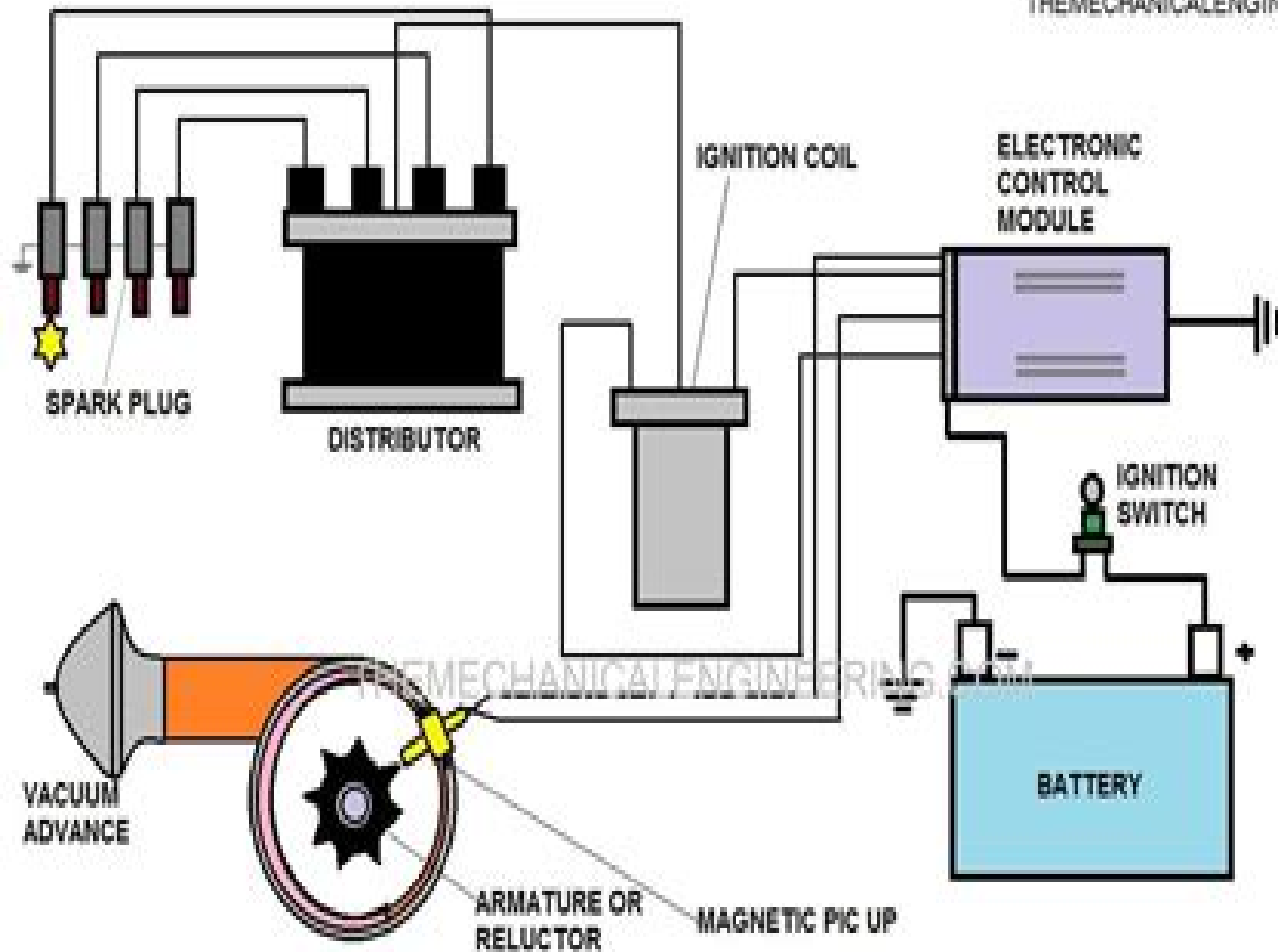
ELECTRONIC IGNITION SYSTEM
